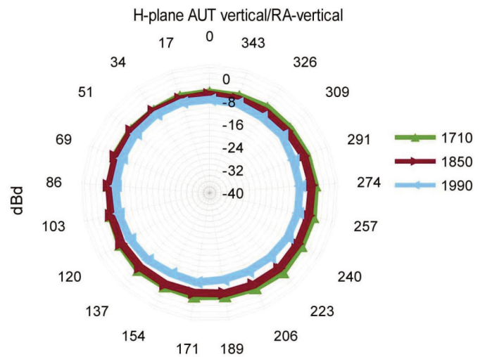
estimated gain (dBd) 1800/1900 MHz band
