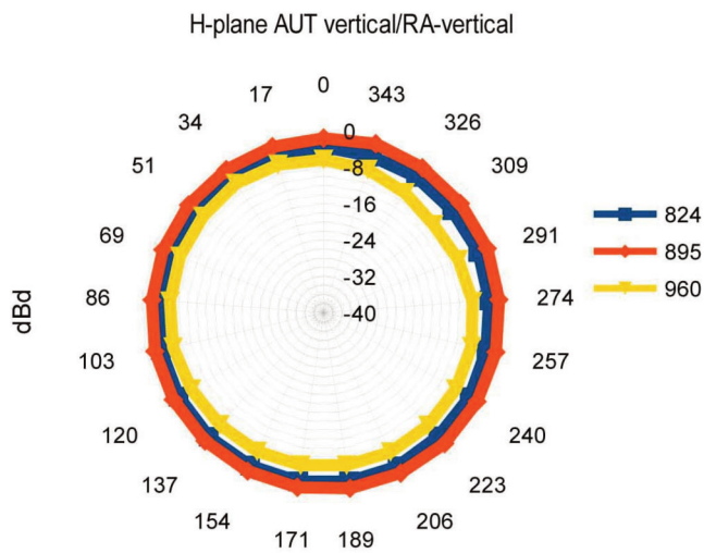
estimated gain (dBd) 850/900 MHz band
