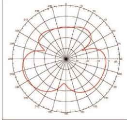
E Plane 2170MHz: 0.72134 dBi
