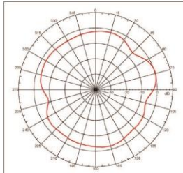
H Plane 2600MHz: -7.49977 dBi
