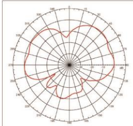
H Plane 824MHz: 1.77902 dBi
