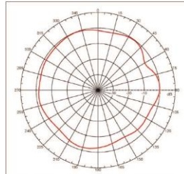
H Plane 1900MHz: -0.03944 dBi
