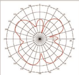
H Plane 900MHz: -2.47165 dBi
