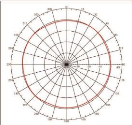
H Plane 2170MHz: 0.020 dBi
