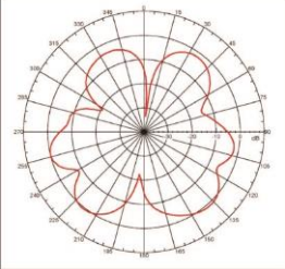
E Plane 2500MHz: 1.04758dBi
