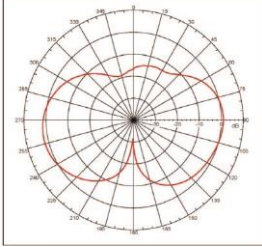
E Plane 1800MHz: 1.76763 dBi
