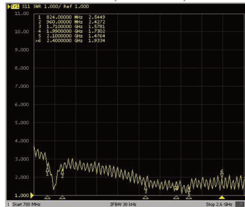
VSWR (Penta Band)
