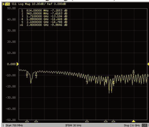
Log Mag (Penta Band)
