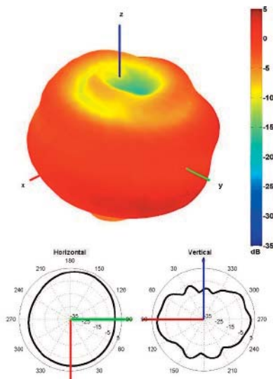
868 MHz Radiation pattern
