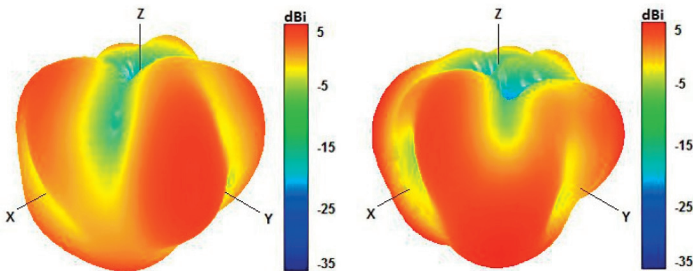
750 and 850 MHz Radiation pattern
