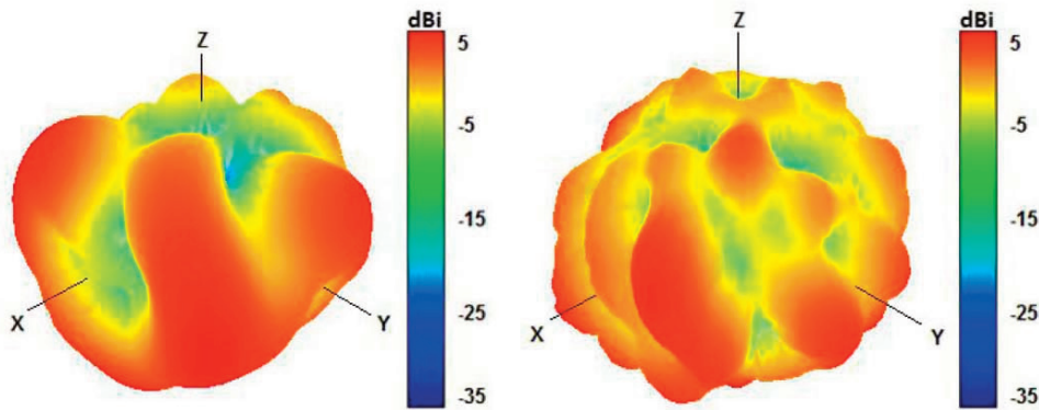
940 and 1750 MHz Radiation pattern
