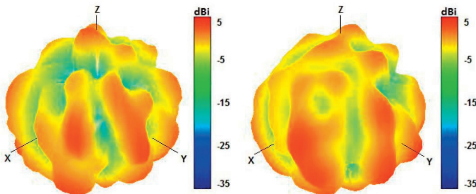
1850 and 1950 MHz Radiation pattern
