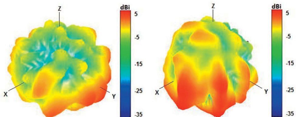
2100 and 2600 MHz Radiation pattern
