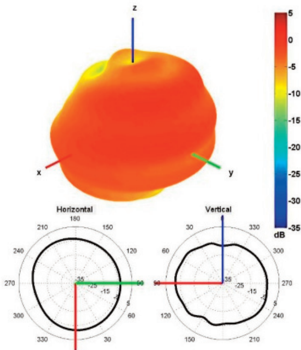
450 MHz Radiation pattern
