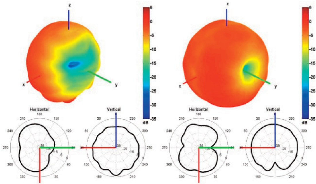
750 and 2500 MHz Radiation pattern
